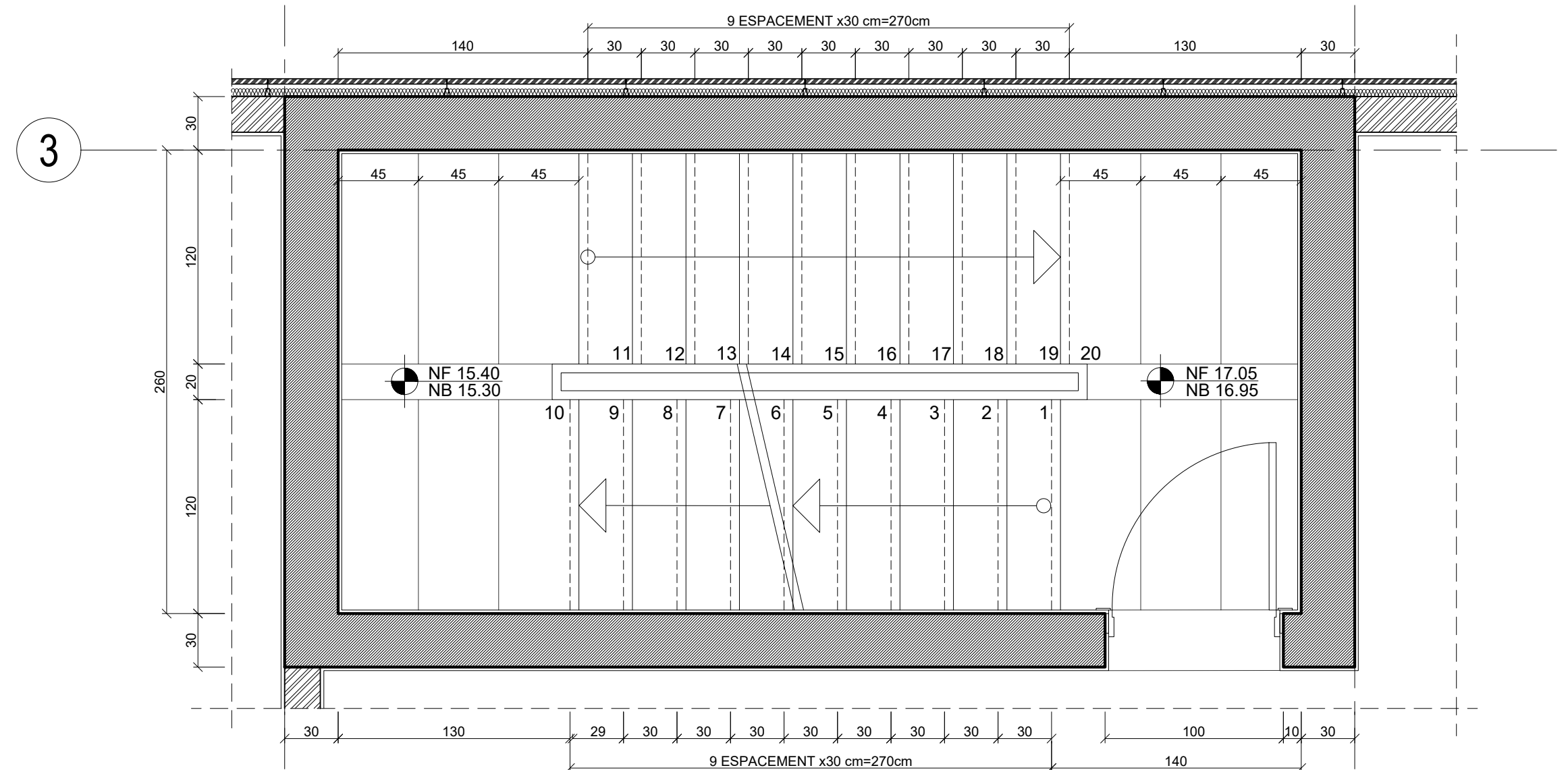
3 - STAIRCASE PLAN TYPICAL LEVEL 1/20
